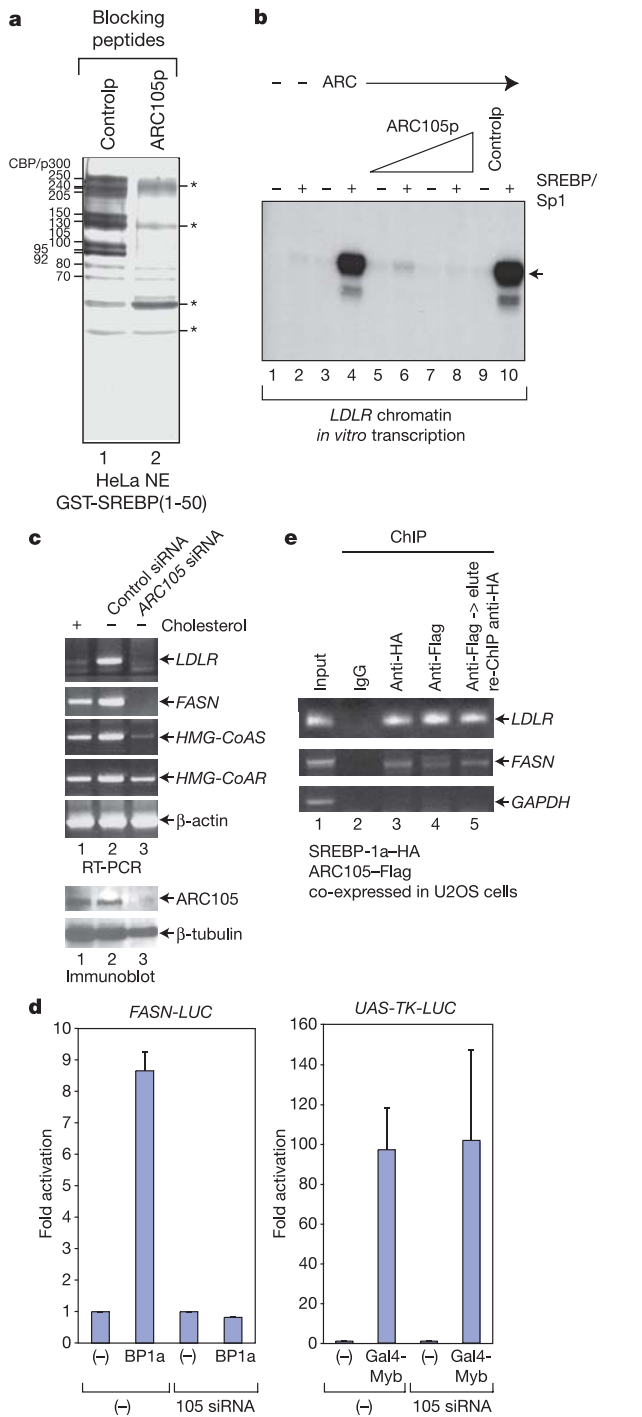
Figure 3 | ARC105 is required for SREBP-dependent transactivation and associates with SREBP target genes in human cells. a , An ARC105 KIX peptide (ARC105p) inhibits binding of both CBP/p300 and the ARC/Mediator co-activator to the GST-SREBP-1a activation domain, whereas a control peptide (Controlp) has no effect. Molecular weights and asterisks are as in Fig. 1a. b , ARC105p inhibited ARC/Mediator-dependent activation by SREBP-1a and Sp1 in an in vitro transcription reaction with LDLR promoter-derived chromatin template. c , ARC105 knockdown by siRNA in HeLa cells results in decreased cholesterol-regulated expression of SREBP target genes, including LDLR , FASN , HMG-CoAS and HMG-CoAR . d , ARC105 RNAi inhibited SREBP-1a-dependent transactivation of a FASN promoter reporter, without affecting Gal4-MybAD transactivation. e , Chromatin immunoprecipitation (ChIP) of SREBP-1a-HA and ARC105-Flag on SREBP target genes in U2OS cells. GAPDH was used as control. Re-ChIP with anti-HA after anti-Flag immunoprecipitation and Flag peptide elution showed that SREBP-1a and ARC105 co-occupy SREBP target genes. Error bars represent s.e.m.
