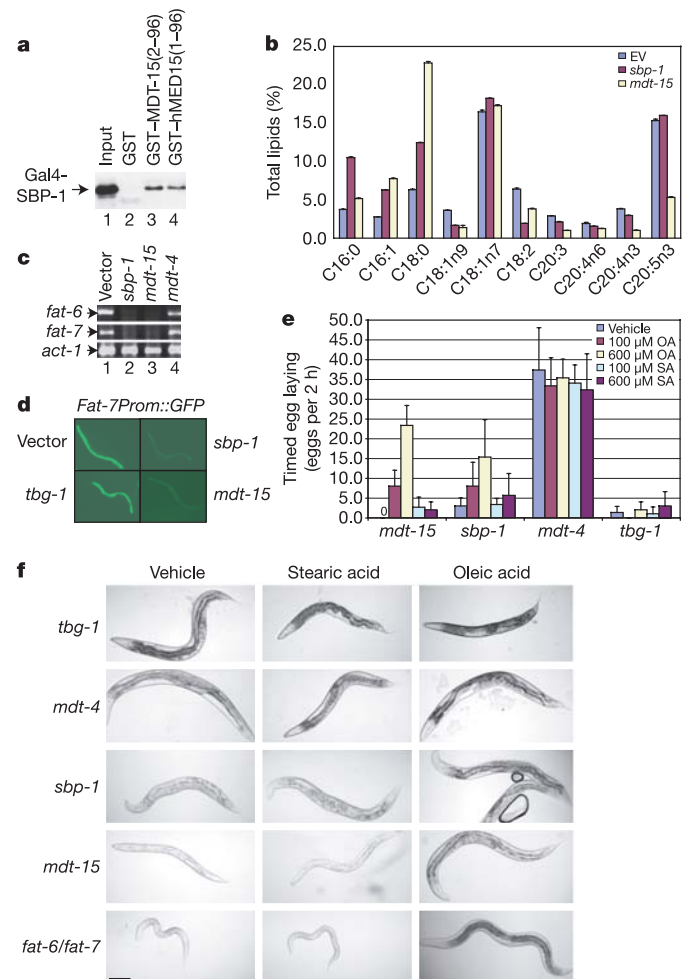
Figure 4 | The C. elegans ARC105 homologue MDT-15 is a critical regulator of C. elegans SREBP (SBP-1) target genes and is required for normal lipid homeostasis. a , The SBP-1 activation domain interacted with the KIX domains of C. elegans MDT-15 and human ARC105. b , Gas chromatography/mass spectrometry analysis revealed altered fatty acid profiles in sbp-1 (RNAi) and mdt-15 (RNAi) nematodes, as compared with empty vector control. c , Transcription of the fat-6 and fat-7 stearoyl-CoA desaturases was strongly decreased upon RNAi of sbp-1 and mdt-15 . d , Intestinal expression of the fat-7 promoter fused to GFP ( fat-7Prom::GFP ) decreased after RNAi of sbp-1 and mdt-15 . e , Dietary addition of oleic acid (OA), but not stearic acid (SA), partially rescued sterility due to mdt-15 and sbp-1 RNAi, while having no effect on controls ( tbg-1 (RNAi) and mdt-4 (RNAi)). f , RNAi of sbp-1 , mdt-15 and fat-6 and fat-7 yielded pale intestines and smaller animals. Dietary addition of 600 \mu M oleic acid, but not stearic acid, darkened the intestines and increased the size of mdt-15 (RNAi), sbp-1 (RNAi) and fat-6/fat-7 (RNAi) nematodes. The scale bar in the lower left panel represents 0.1 mm. Error bars represent s.e.m.
